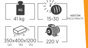
FK 02 FESTİNA KLİPS MAKİNESİ FESTINA CLIPS MACHINE
