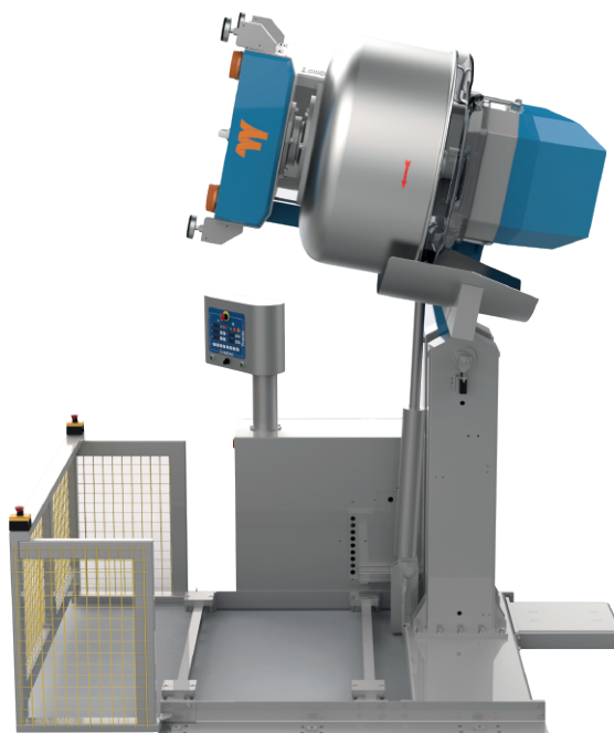
SKKD SABİT KAZANLI KALDIR-DEVİR TILT OVER SİRİRAL MIXER
