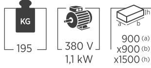
HKC 01 HAMUR KONİK ÇEVİRME MAKİNESİ CONICAL ROUNDING MACHINE
