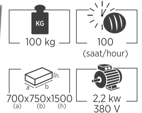
PM 01 PUDRA ŞEKERİ MAKİNESİ POWDERED SUGAR MACHINE
